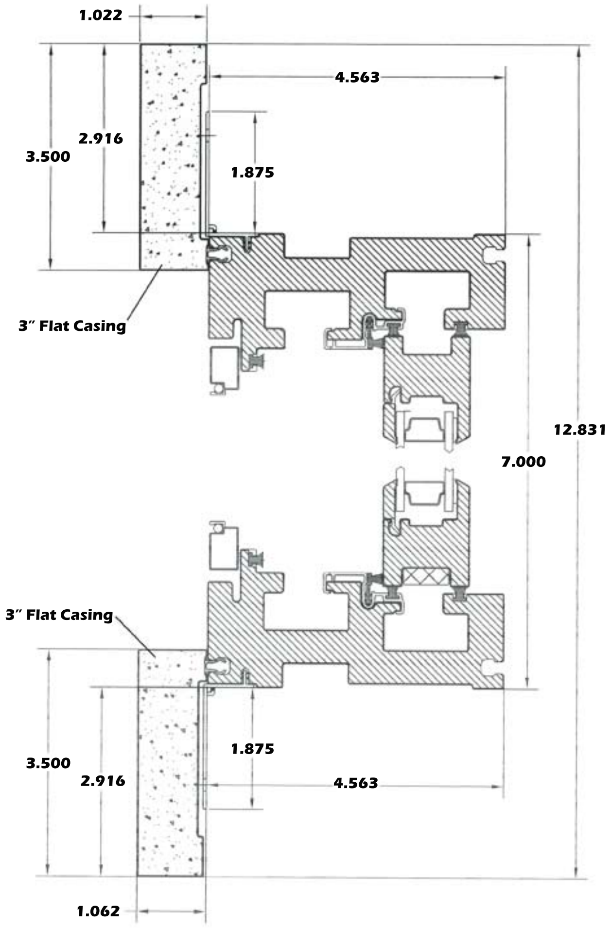
Double Hung Horizontal 3" Flat Casing
