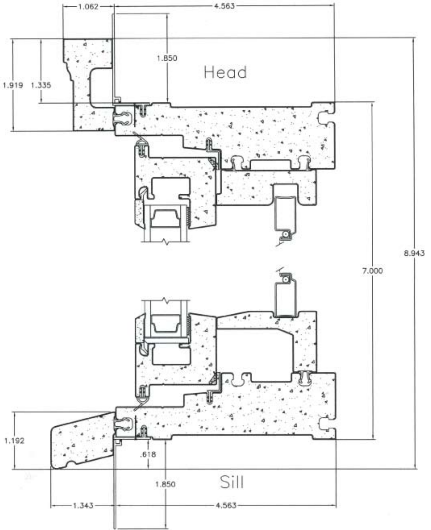
Casement Vertical View Brickmold at Head & Sill Nose
