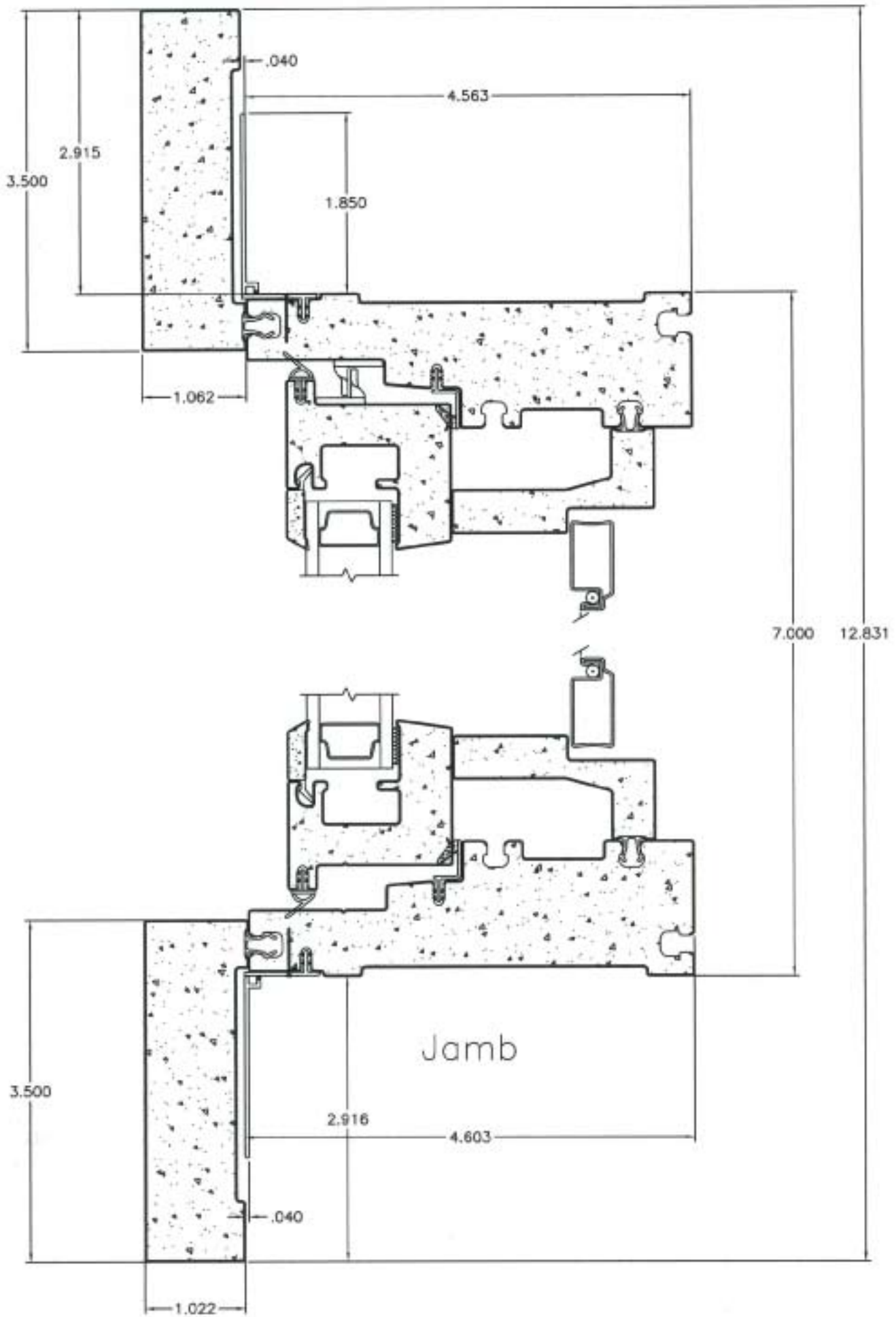
Casement Horizontal View 3½" Flat Casing on Jambs
