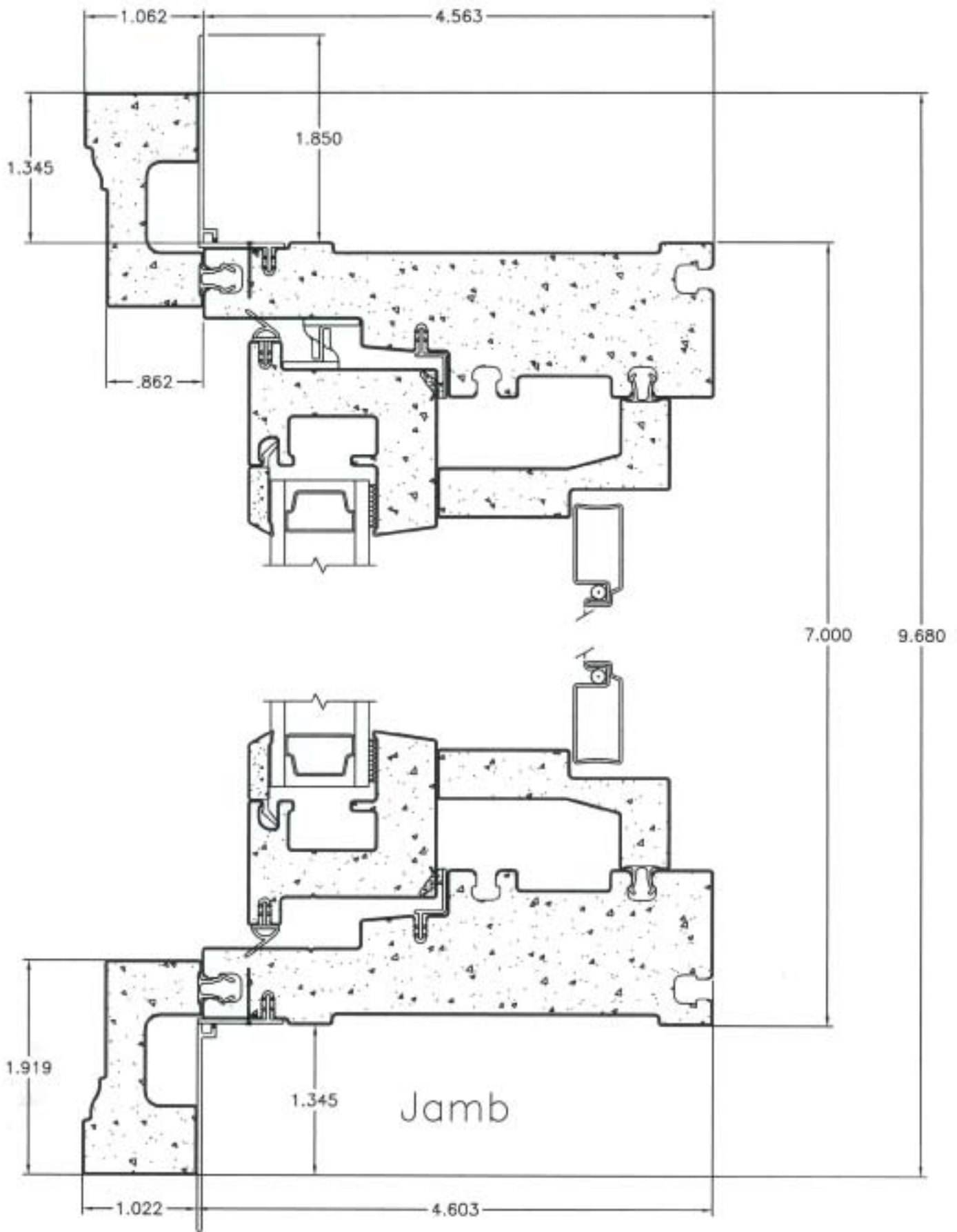
Casement Horizontal View Brickmold on Jambs
