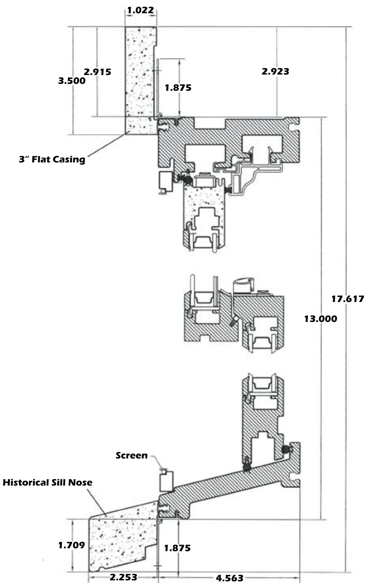
Double Hung Jamb - Vertical 3" Flat Casing and Historical Sill Nose
