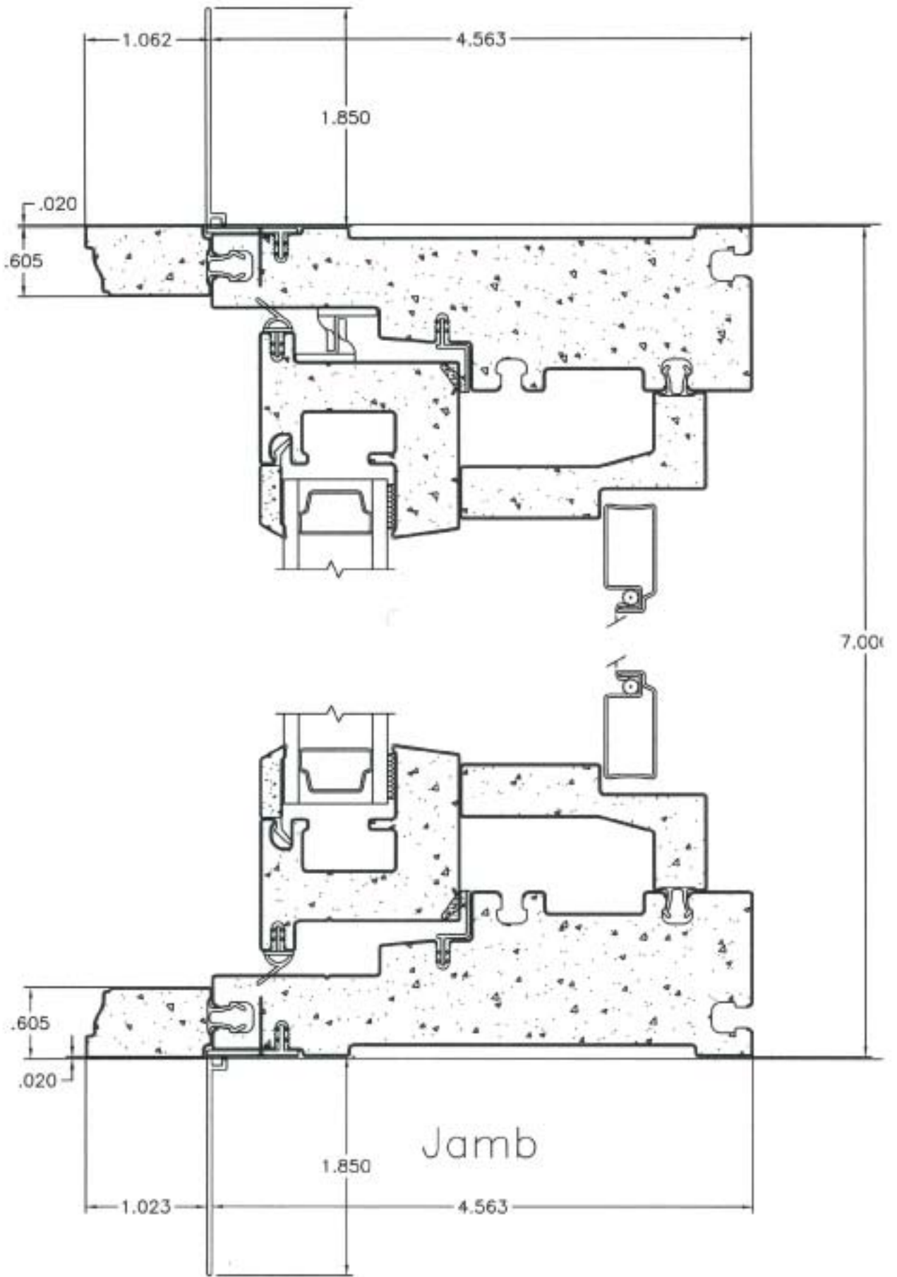
Casement Horizontal View 1: Curbing on Jambs
