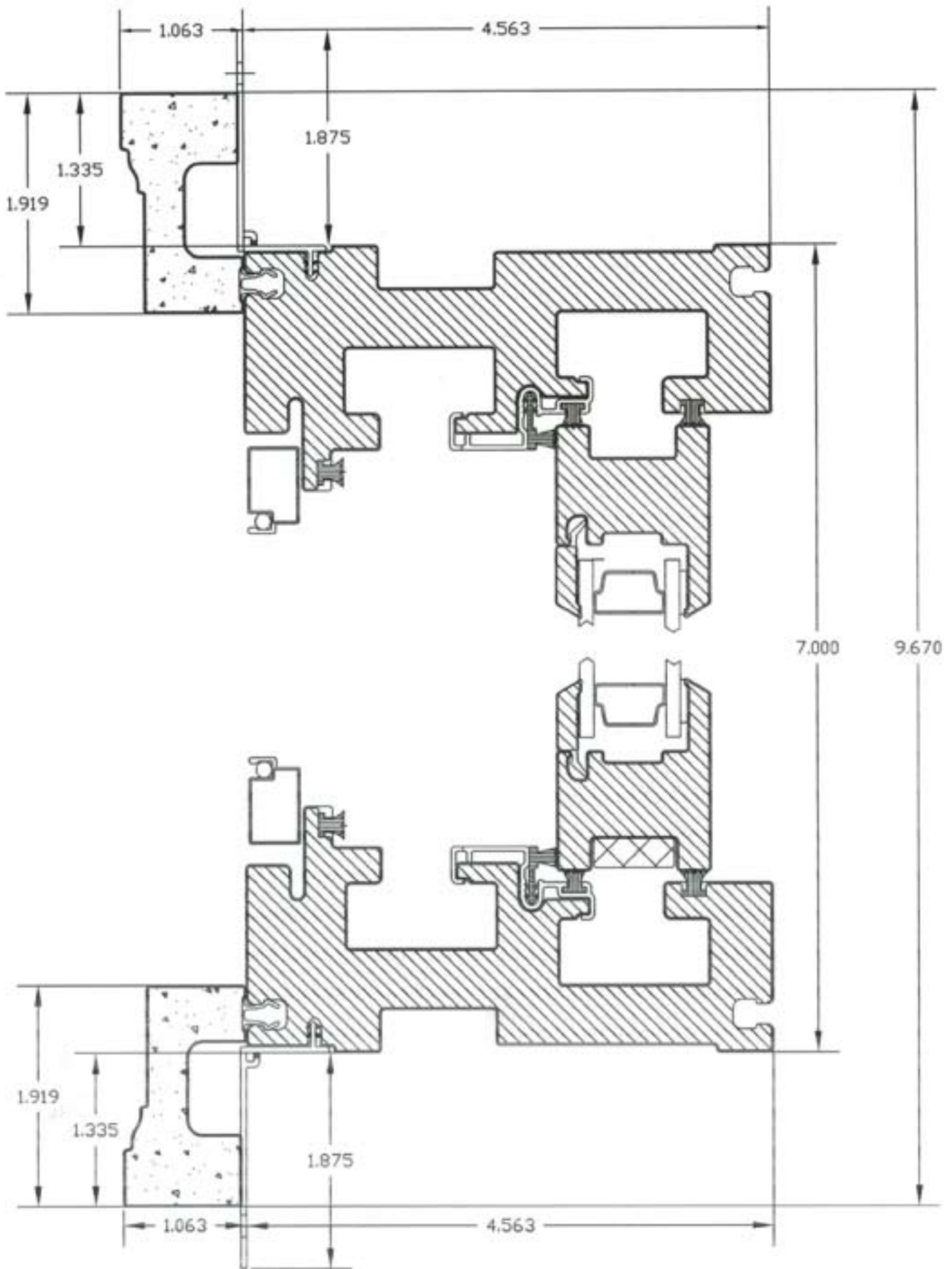
Double Hung Horizontal View Brickmold on Jambs
