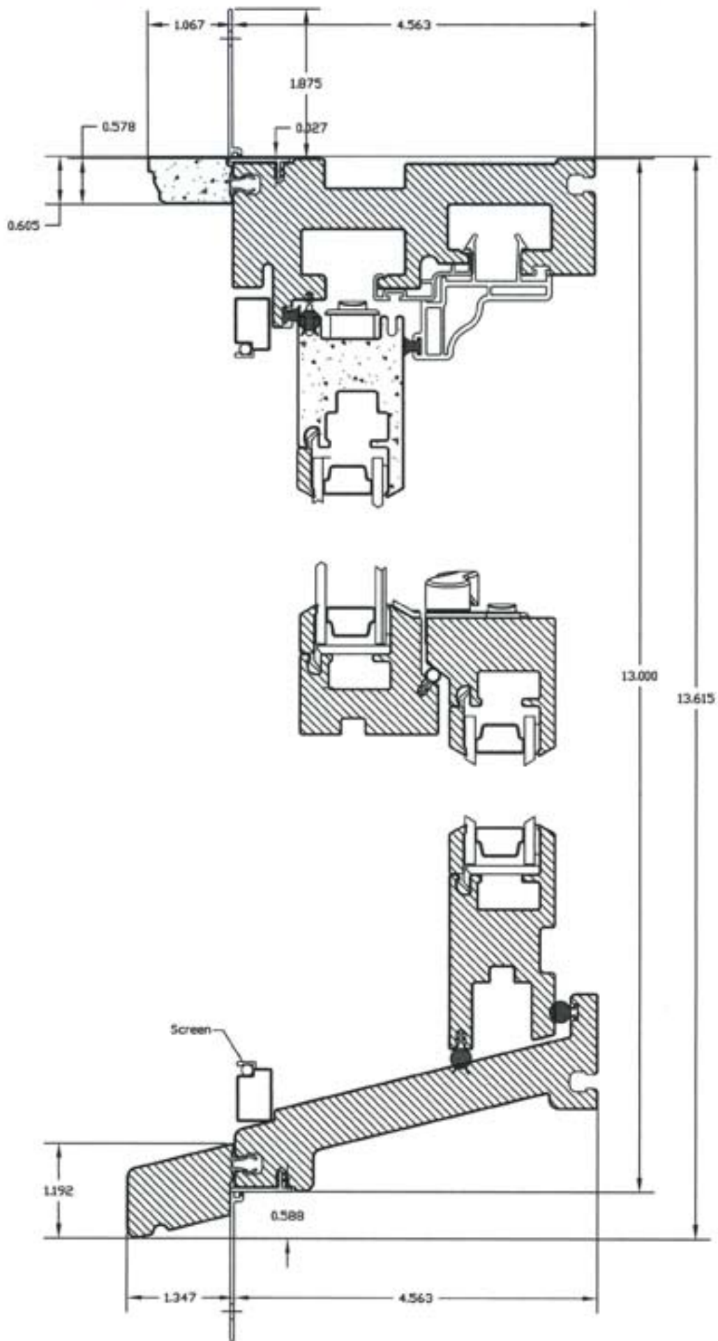
Double Hung Vertical View 1" Curbing at Head/Sill Nose
