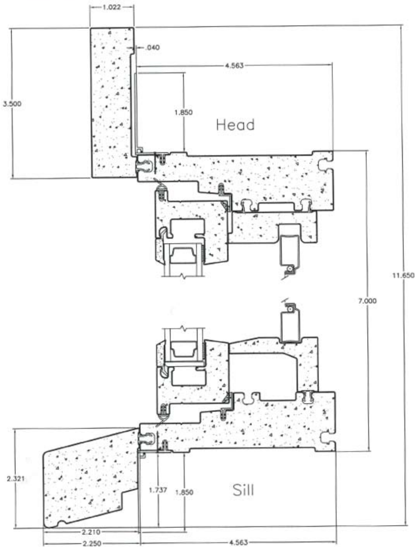
Casement Vertical View 3½" Flat Casing at Head & Historical Sill Nose
