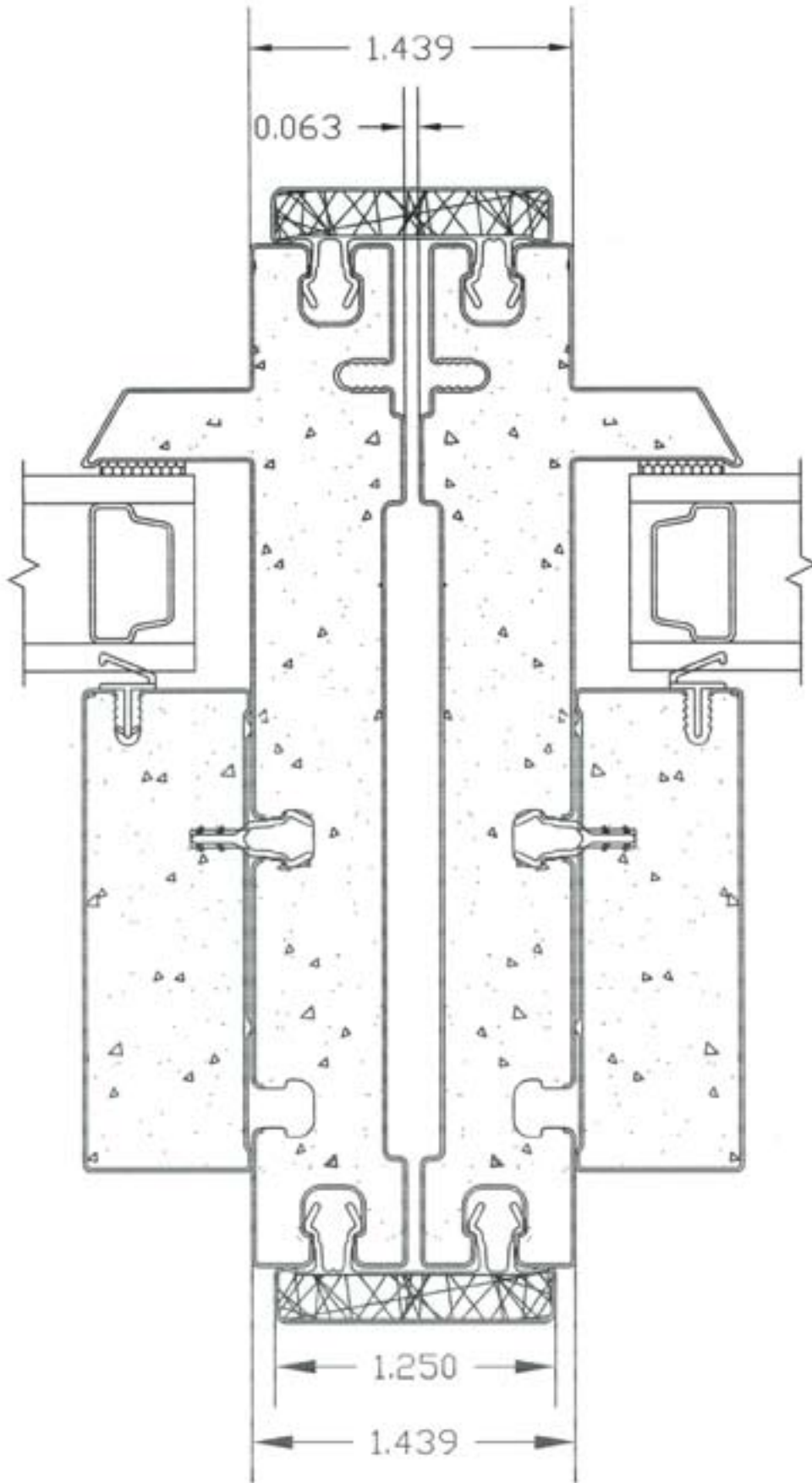
Mullion Detail Double Hung & Direct Set Picture Window
